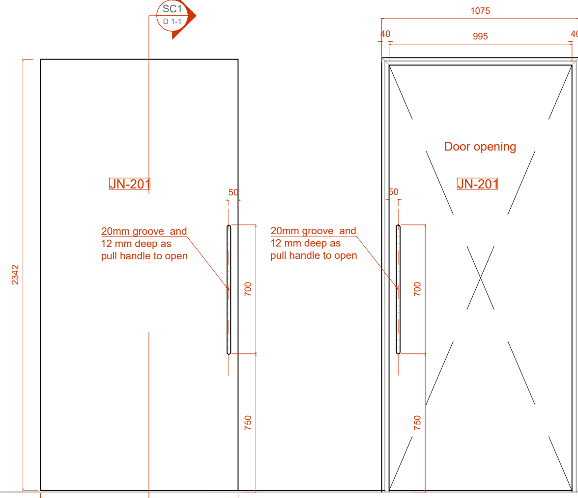
Section outside view Inside view
